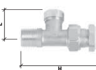
Straight lock shield valve for copper, PEX or multilayer pipe with GE System
